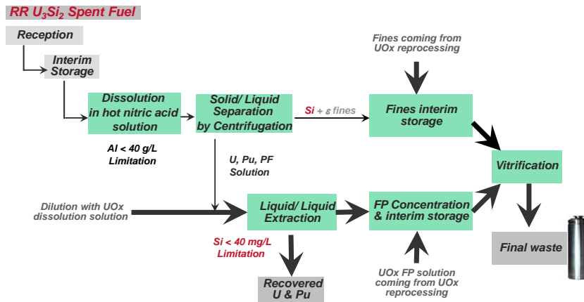
Fig 2. Process diagram for Silicide fuels reprocessing in New AREVA La Hague plant
