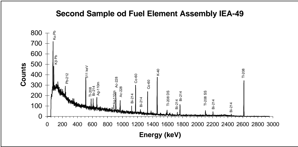
Figure 9 - Sipping Water Sample Gamma-Ray Spectrum
