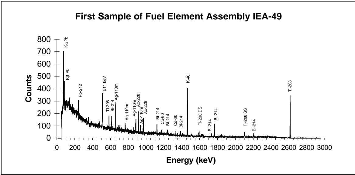
Figure 8 - Sipping Water Sample Gamma-Ray Spectrum
