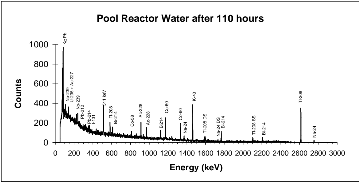
Figure 5 - Pool Water Sample Gamma-Ray Spectrum
