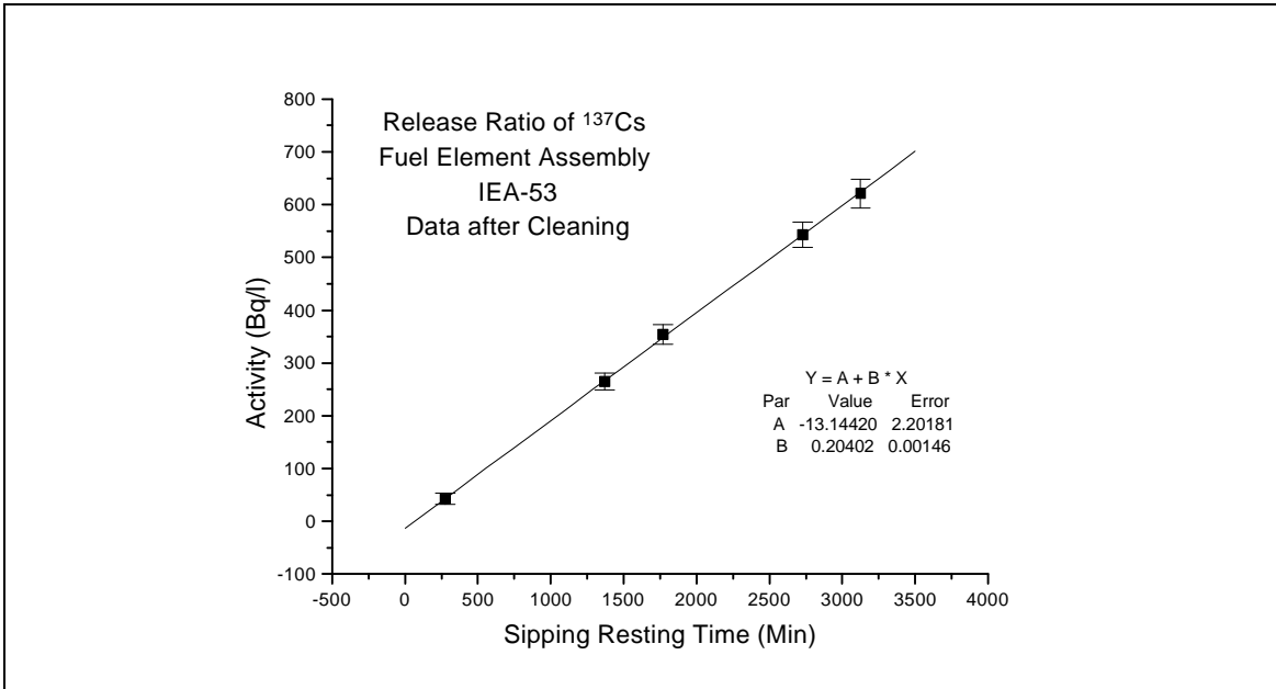
Figure 13 - ^{137}\text{Cs} Leaking Rate Determination
