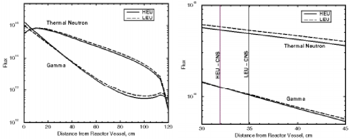
Figure 3. Unperturbed Reflector: HEU and LEU Thermal Neutron and Gamma Fluxes
