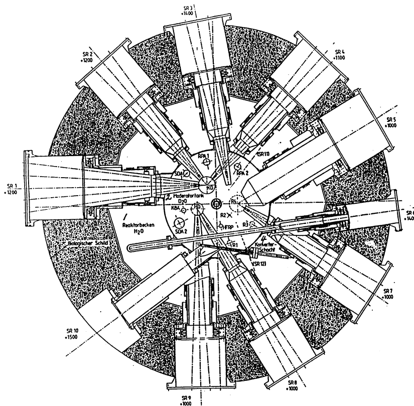
Figure 1: Horizontal Section Through TUM FRM-II (Reproduced from Figure 4 of Ref. 5)
