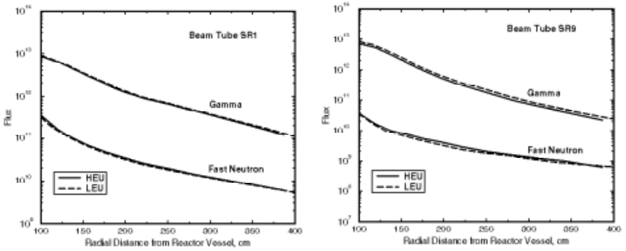
Figure 6. Fast Neutron and Gamma Fluxes Inside Beam Tubes
