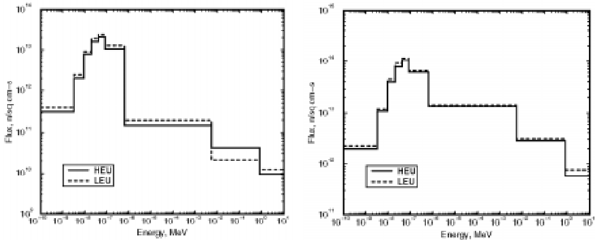
Figure 5. Spectra at the Tip of Beam Tubes SR 5 (left) and SR 8 (right)
