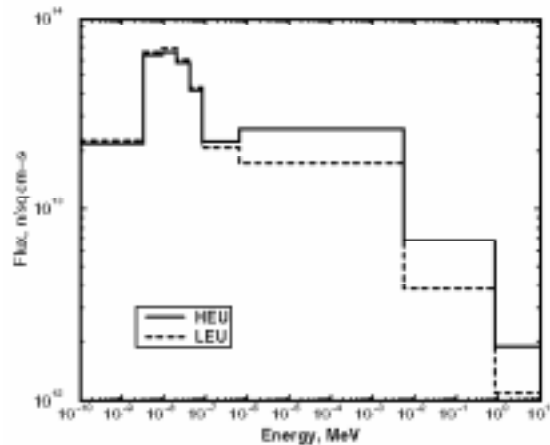
Figure 4: Spectra at the Cold Neutron Source
