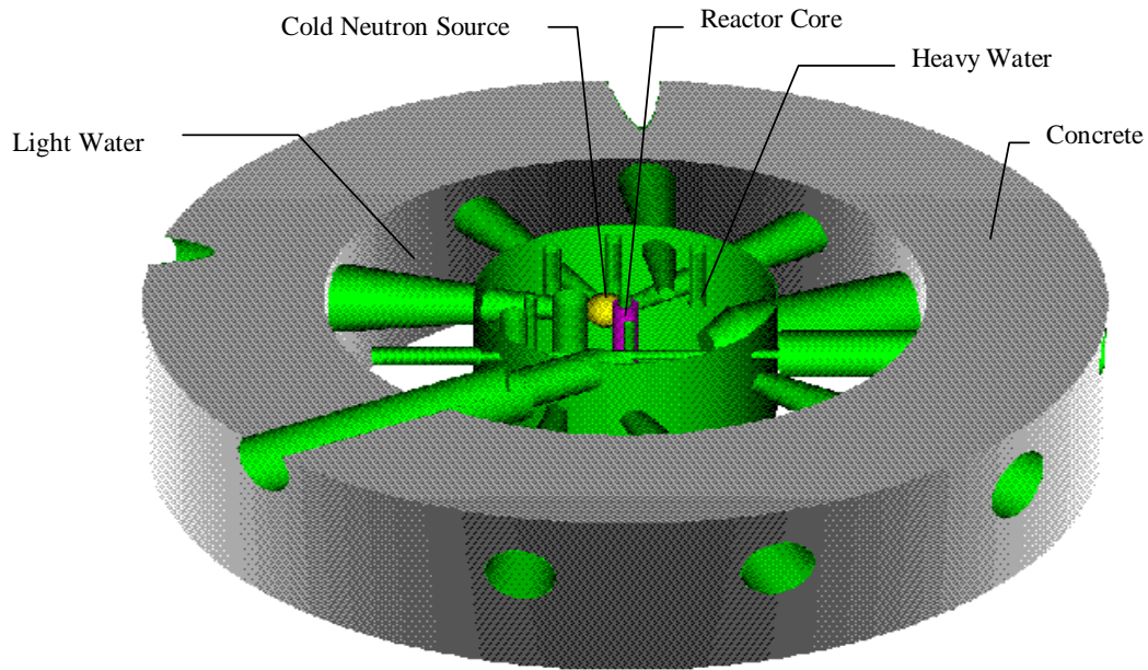
Figure 2. View of Model Used in MCNP Analyses
