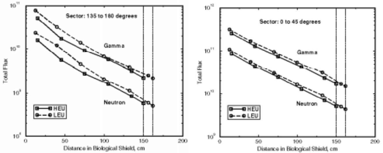
Figure 7. Total Neutron and Gamma Fluxes in Different Sectors of the Biological Shield (Biological Shield Thickness: 150 cm for HEU; 162 cm for LEU)
