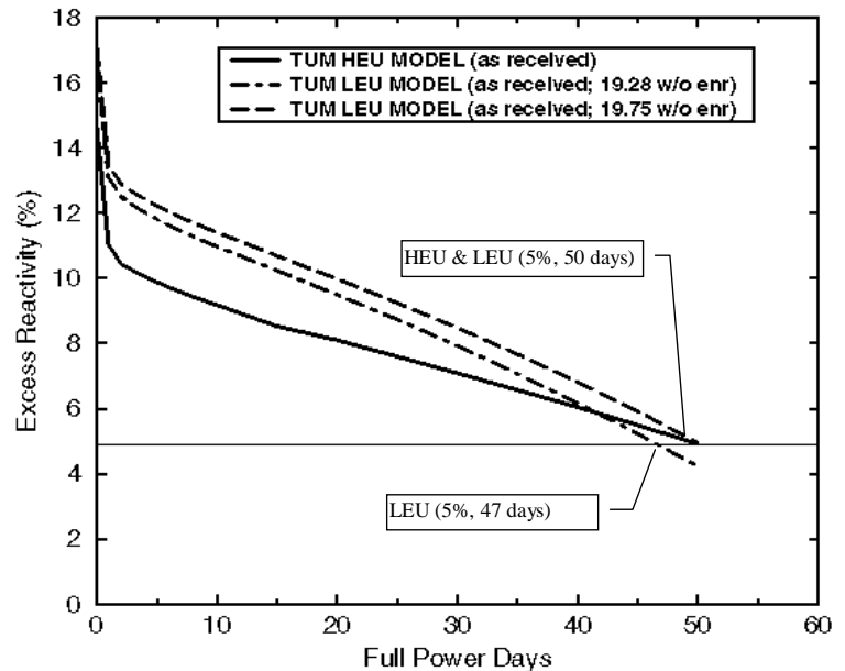
Figure 8. Reactivity Rundown for TUM Models of the FRM-II HEU Design and the ANL Alternative LEU Design
