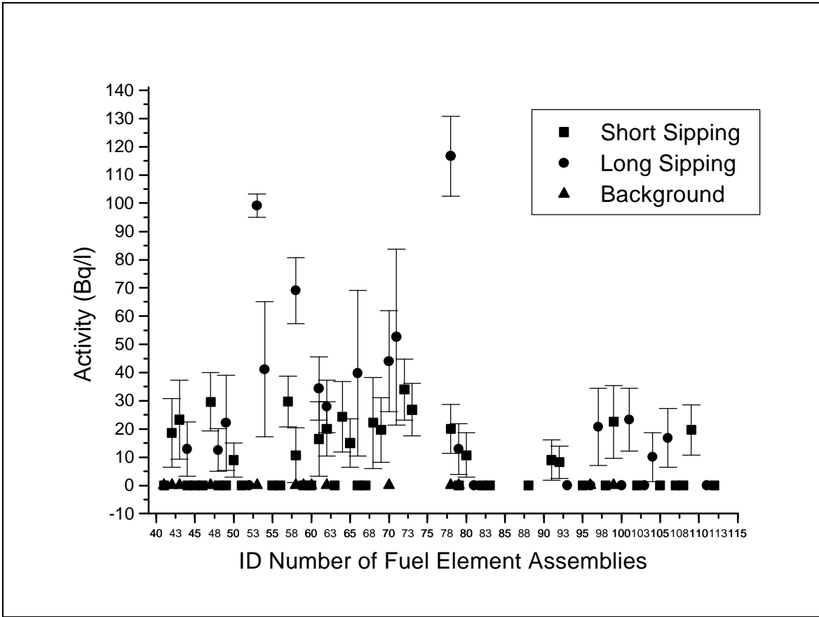
Figure 7 - Fuel Assemblies Sipping Water Samples Activity Results
