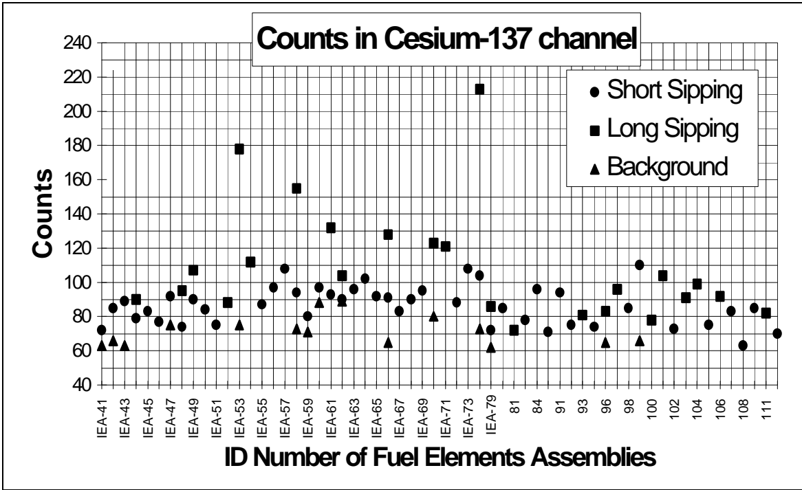
Figure 6 - Fuel Assemblies Sipping Water Samples Counting Results
