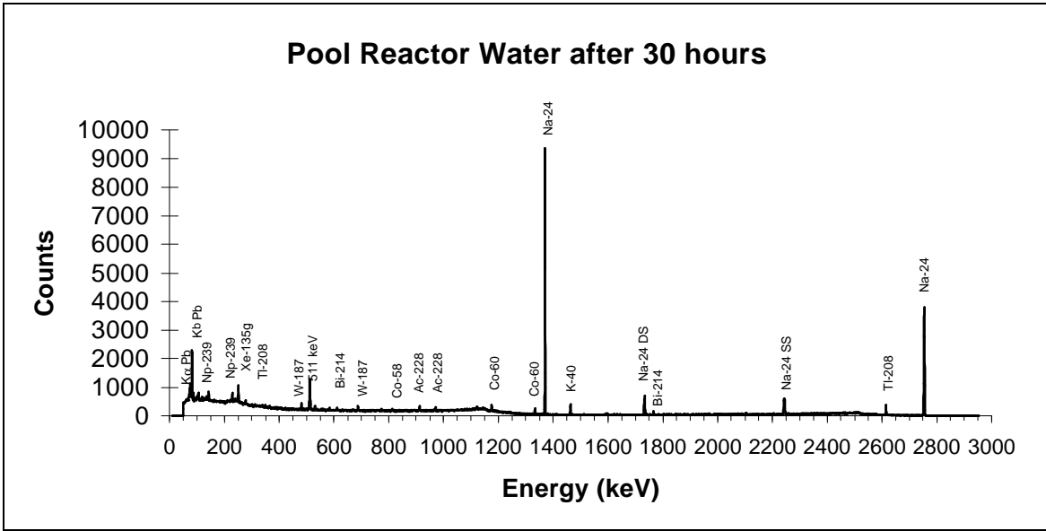
Figure 4 - Pool Water Sample Gamma-Ray Spectrum
