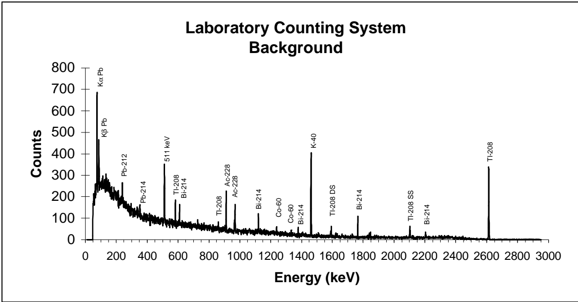
Figure 3 - Laboratory System Background Gamma-Ray Spectrum
