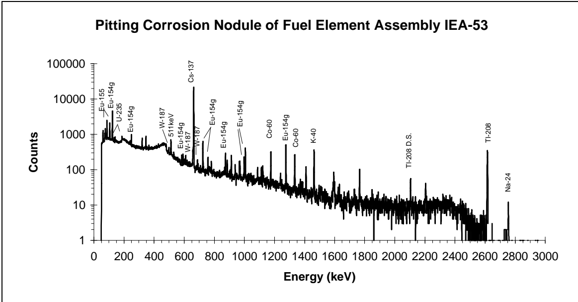
Figure 15 - Pitting Corrosion Nodule-Gamma Ray Spectrum
