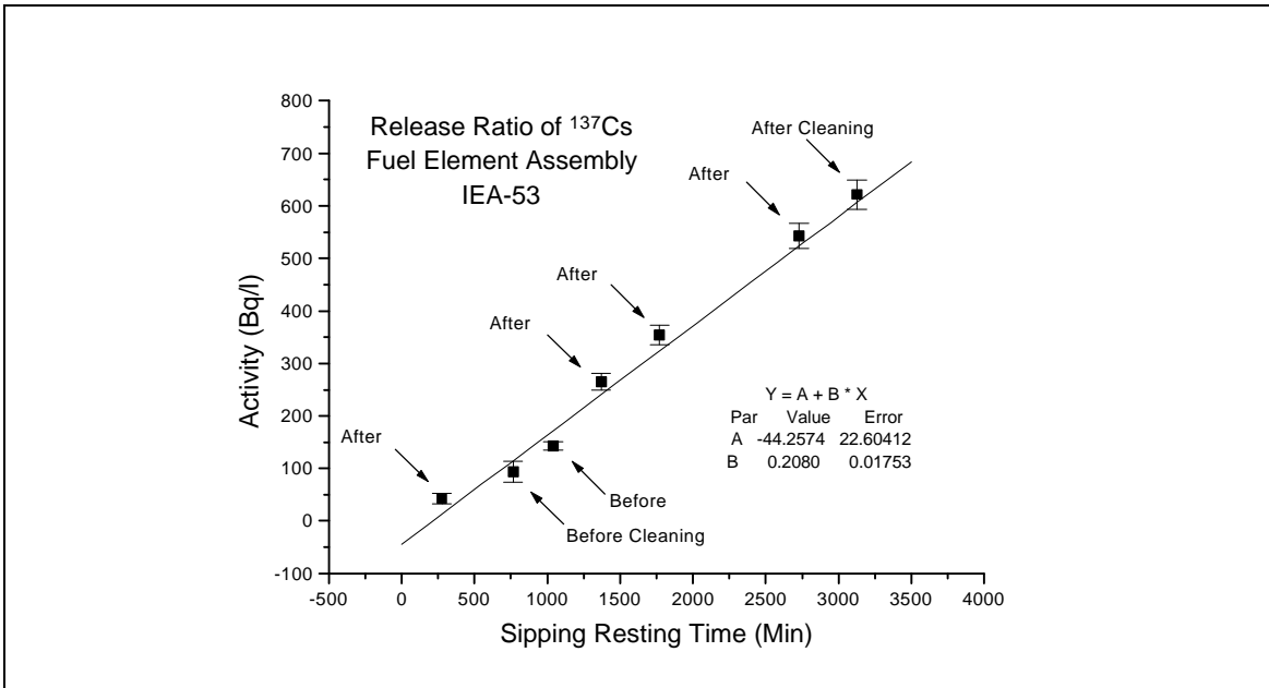
Figure 14 - ^{137}\text{Cs} Leaking Rate Determination
