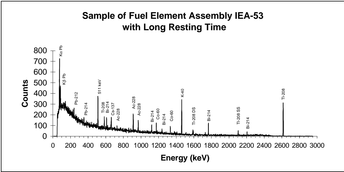
Figure 11 - Sipping Water Sample Gamma-Ray Spectrum
