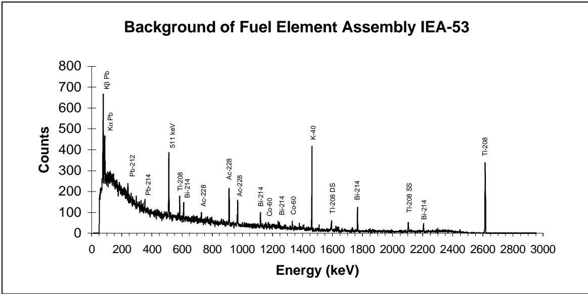
Figure 10 - Sipping Water Sample Gamma-Ray Spectrum
