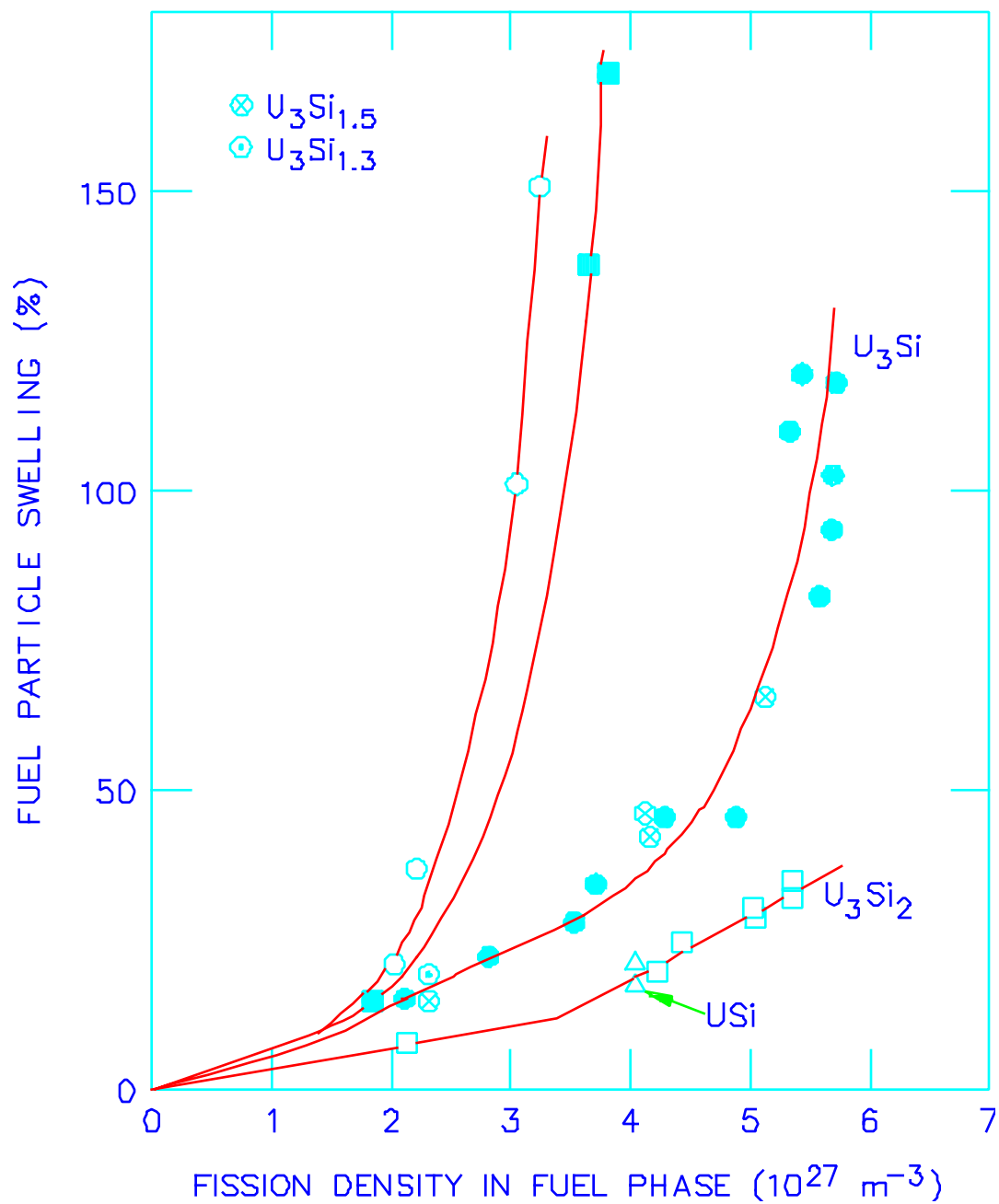
Fig. 1. Swelling of LEU fuel particles in experimental aluminum dispersion fuel plates irradiated in the ORR.
