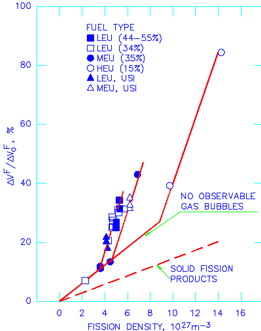
Fig. 2. Swelling of U_3Si_2 of various enrichment and fuel dispersion loadings as a function of fission density (USi data included).
